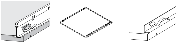
Clip-In Suspension
